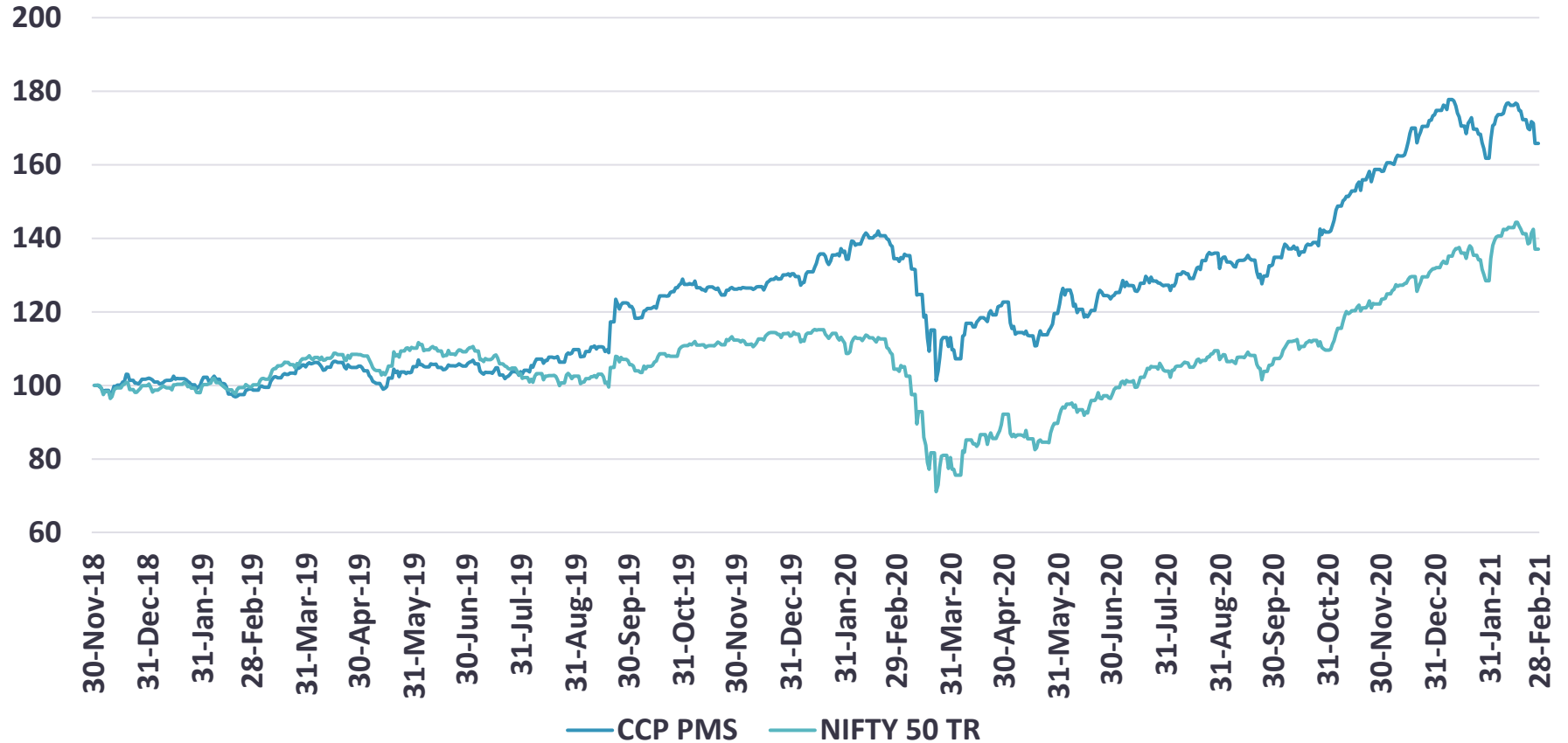
CCP v/s NIFTY50 performance
